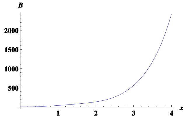
Plot of the magnetic field ( B ) for density ratio n_{ih} = 0.322n_e and n_{il} = 0.677n_e for simple slab geometry. The scale parameters are \lambda_1 = 2.0363 , \lambda_2 = 4.79852 + 1.444 i , and \lambda_3 = 4.79852 - 1.444 i .
