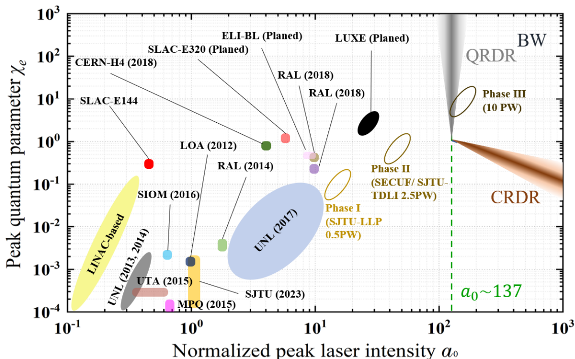
FIG. 5. The relevant international experimental progress and proposals.
