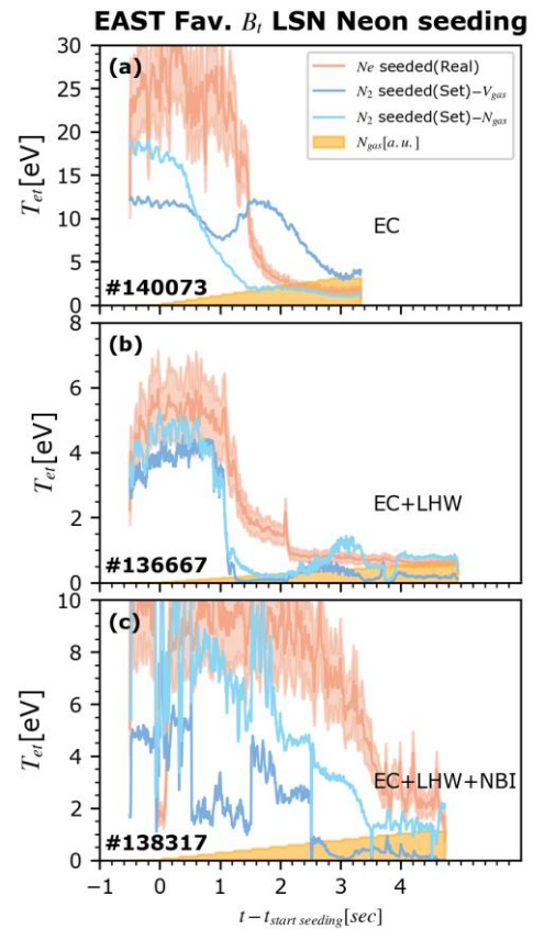
Figure 2 Validation of the Underlying Physics of the Model with Neon seeding scenarios.
